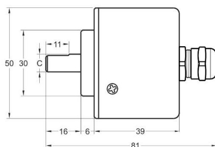
Shaft Type / Axial
